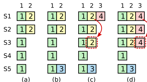
Figure 8: A time sequence showing why a leader cannot immediately make commitment decisions about log entries from older terms. In (a) S1 is leader and has partially replicated the log entry at index 2; then S1 crashes. In (b) S5 has been elected leader for term 3 with votes from S3, S4, and itself; it accepts a different entry at log index 2, but crashes before replicating it. In (c) S1 has been elected leader again, with votes from S2, S3, and S4; after accepting a log entry at index 3, it has just replicated index 2 to S3. At this point, the log entry from term 2 has been replicated on a majority of the servers, but it is not committed: S5 could still be elected leader of a future term (with votes from S2, S3, and S4) and overwrite the entry with its own entry from term 3. In (d) S1 has replicated an entry from its current term on a majority of the servers. This entry is committed (S5 can no longer acquire enough votes to be elected leader), and all preceding entries in the log are now committed as well.
