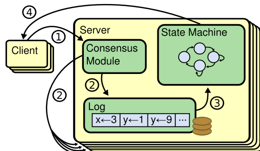
Figure 1: Replicated state machine architecture. The consensus algorithm manages a replicated log containing state machine commands from clients. The state machines process identical sequences of commands from the logs, so they produce the same outputs.
