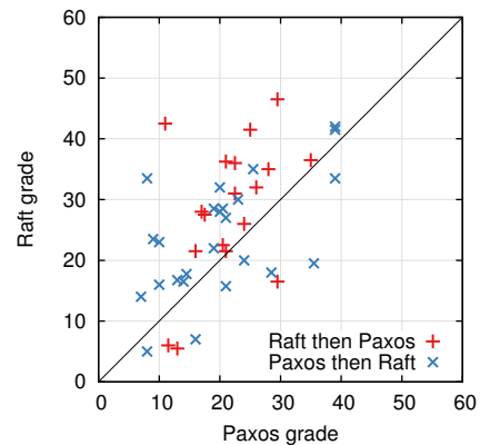
Figure 13: A scatter plot comparing 43 participants’ performance on the Raft and Paxos exams. Points above the diagonal (33) represent participants who scored higher for Raft.
