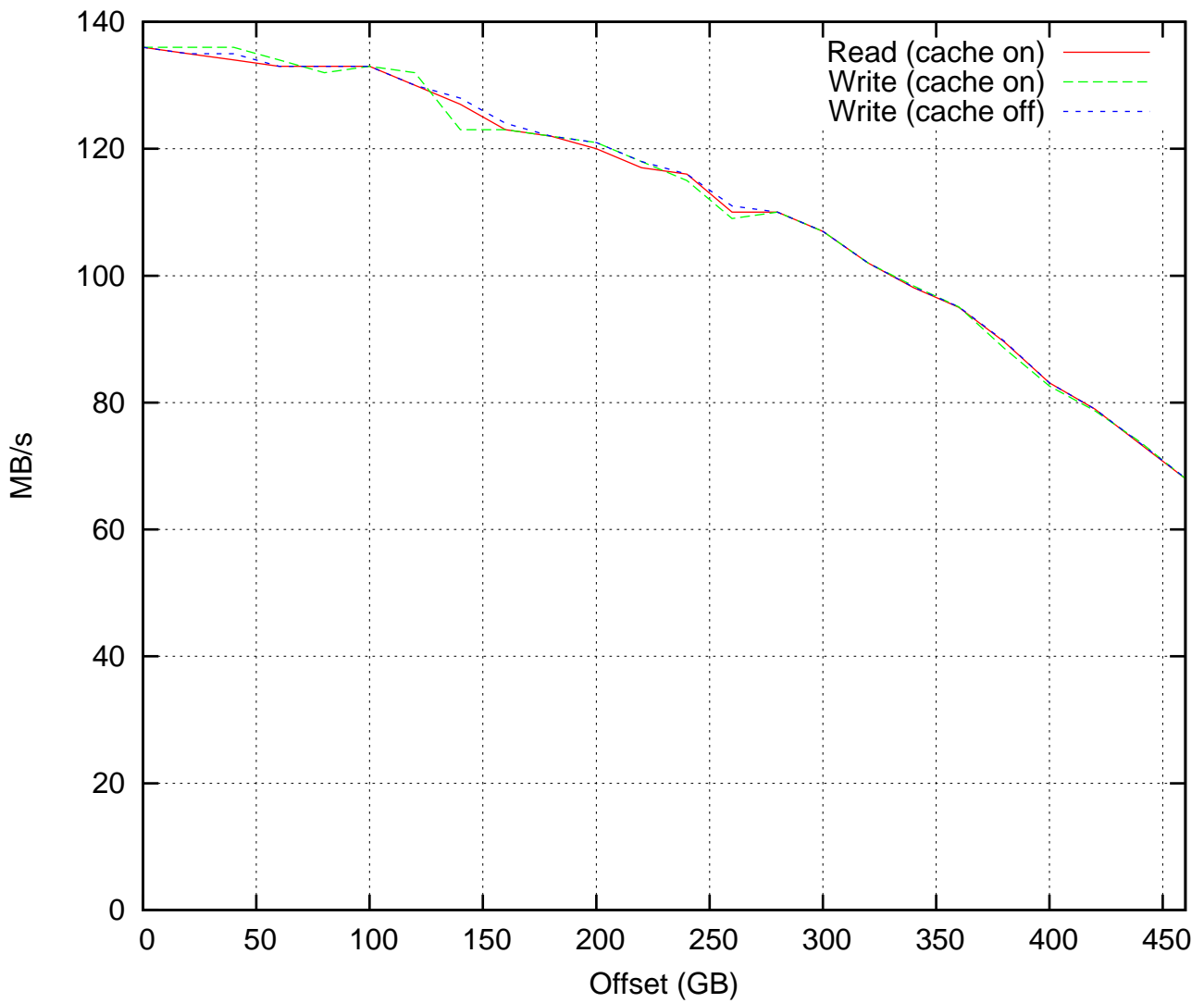
ST3500514NS Sequential Disk Bandwidth
