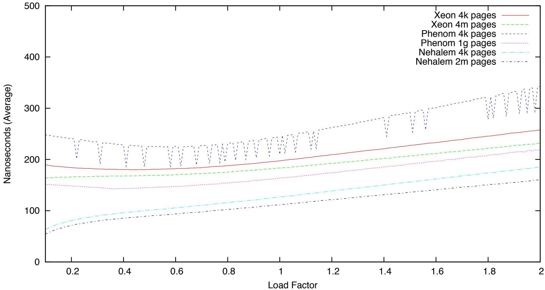
Hash Table Lookup Performance - 12e6 Keys
