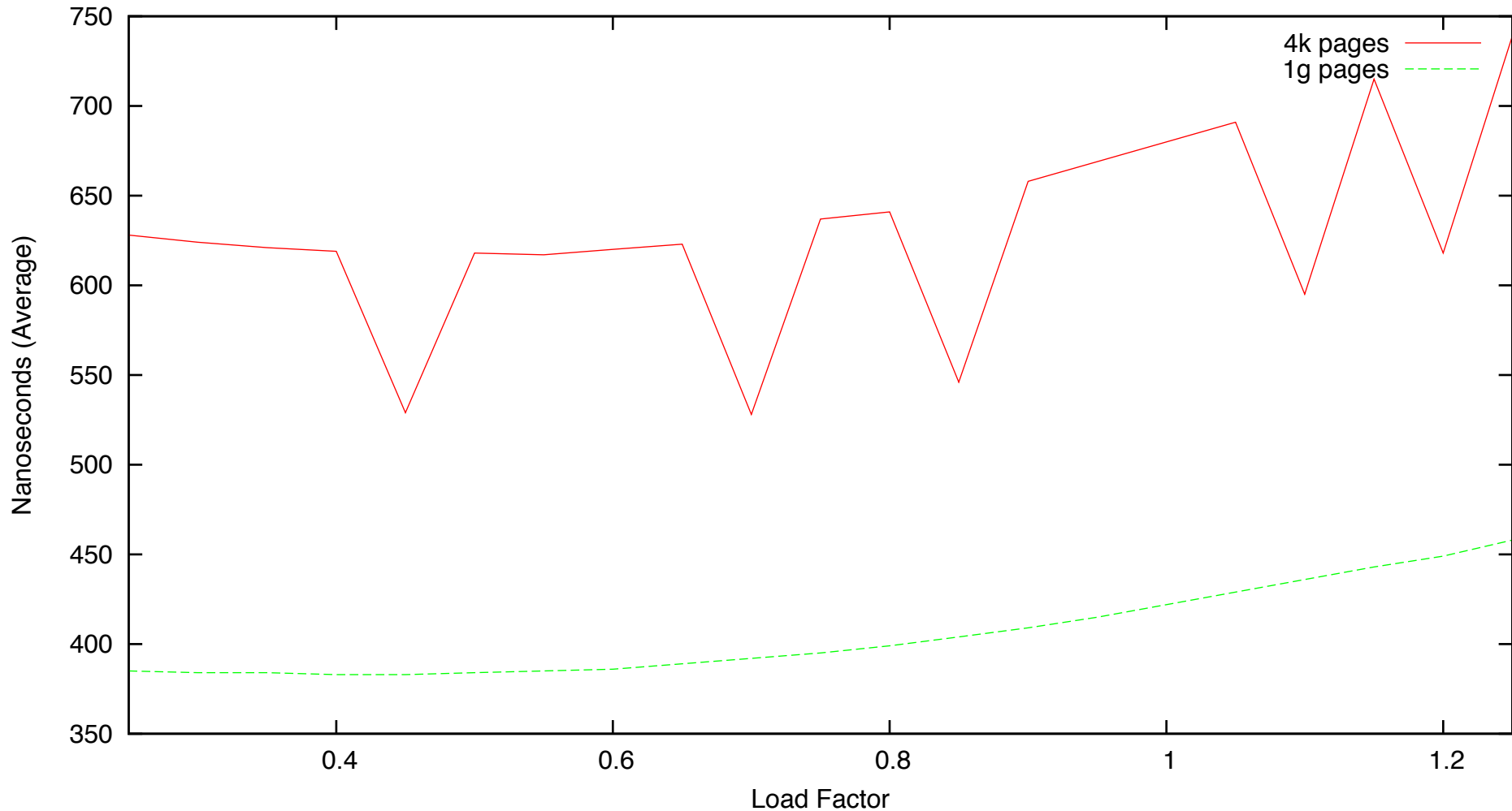
Hash Table Lookup Performance - 30e6 Keys
