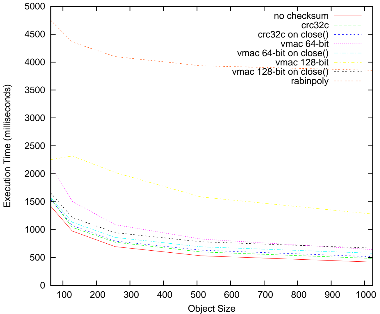
recoverSegment Checksum Performance (no backups, 80x8MB segments)
